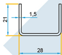
S-634TRE15 Renfort dormant
