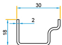
S-634TRE03B Renfort dormant
