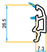
PR.OC.29.BL/511.3 Parcloses double vitrage 16mm
