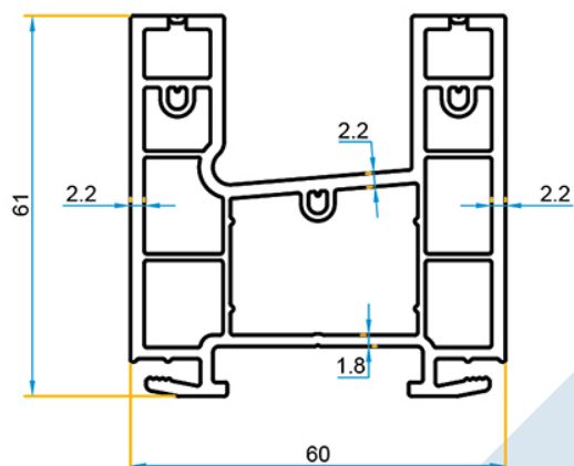
PR.OC.21.BL/222 Dormant standard Blanc
