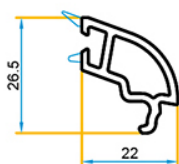
PR.OF.12.BL/511 Parcloses double vitrage 16mm
