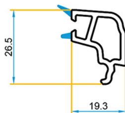
PR.OC.29.BL/511.3 Parcloses double vitrage 16mm
