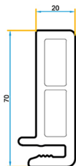
PR.FC.98.BL COUVRE JOINT
